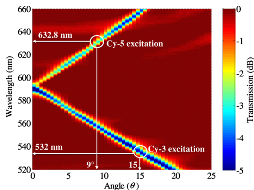
FIG. 4. (Color online) Measured dispersion diagram for the PC used in this study by RCWA. Resonance for the enhanced excitation for the TM mode is \theta \sim 9^\circ for Cy-5 excitation and \theta \sim 15^\circ for Cy-3 excitation.
