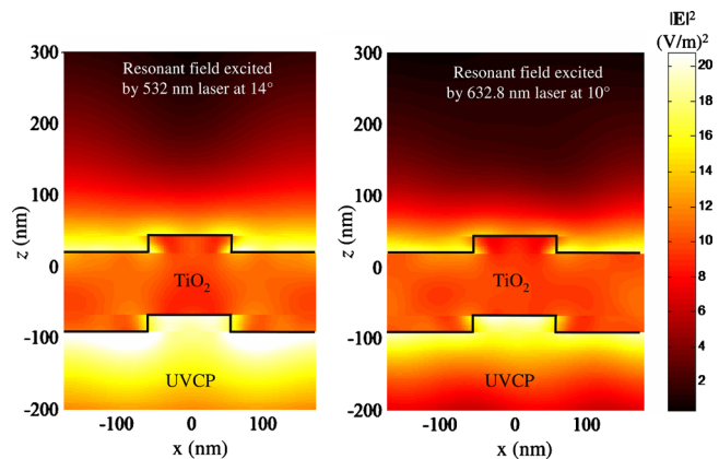
FIG. 3. (Color online) Simulated near field distribution for the PC used in this study by RCWA at \lambda=532 nm and \lambda=633 nm.
