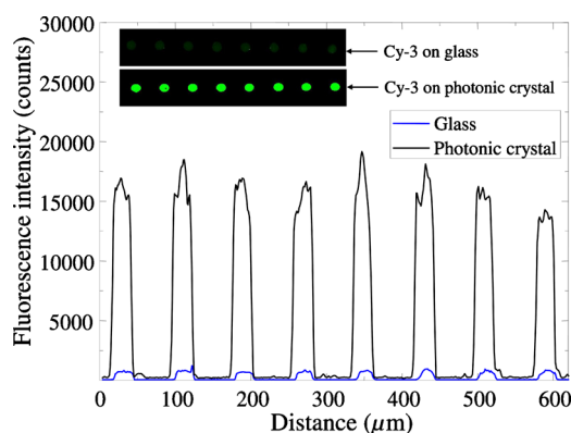
FIG. 6. (Color online) Intensity profile as a function of distance for a line of fluorescent image pixels profiling spots of Cy-3 conjugated streptavidin for both the glass slide and the PC under normal incidence illumination. The scanned images are shown in insets.
