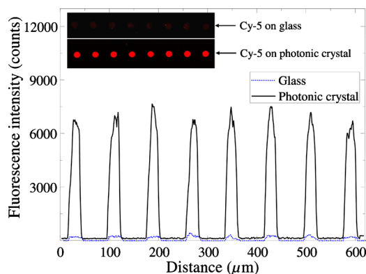
FIG. 5. (Color online) Intensity profile as a function of distance for a line of fluorescent image pixels profiling spots of Cy-5 conjugated streptavidin for both the glass slide and the PC under normal incidence illumination. The scanned images are shown in insets.
