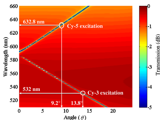
FIG. 2. (Color online) Simulated dispersion diagram for the PC used in this study by RCWA. Resonance for the enhanced excitation for the TM mode is \theta \sim 9.2^\circ for Cy-5 excitation and \theta \sim 13.8^\circ for Cy-3 excitation.
