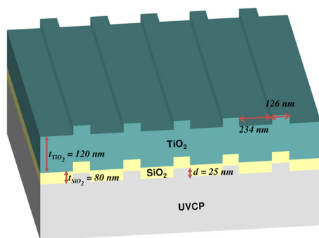
FIG. 1. (Color online) Cross-sectional diagram (not to scale) of the PC. The dimensions are as follows: \Lambda=360 nm, grating depth d=25 nm, \text{SiO}_2 thickness t_{\text{SiO}_2}=80 nm, and \text{TiO}_2 thickness t_{\text{TiO}_2}=120 nm. The grating width is 35% of the period.
